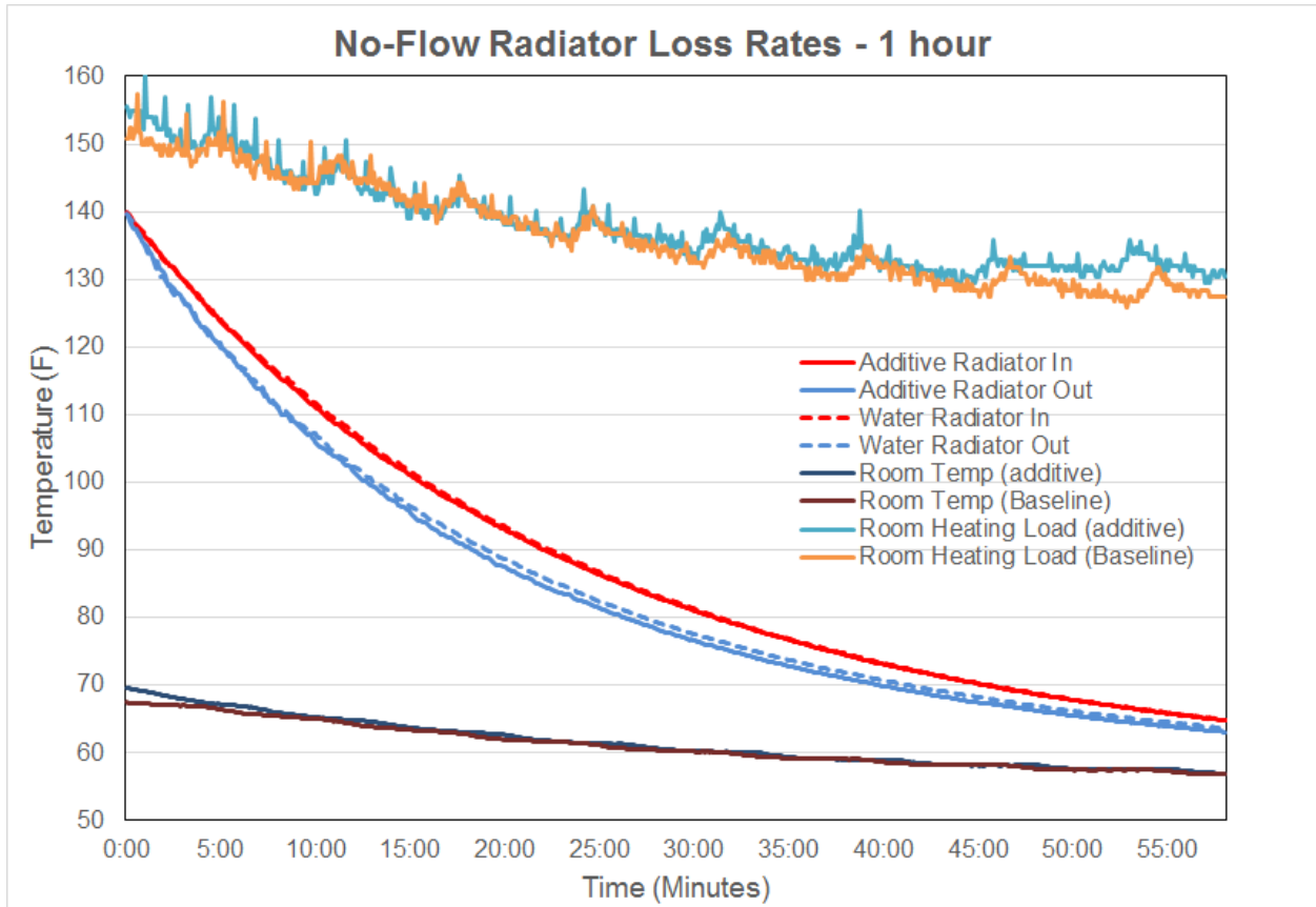
Figure 2: Temperature Decay with Additive Compared to Water at Zero Flow Rate
