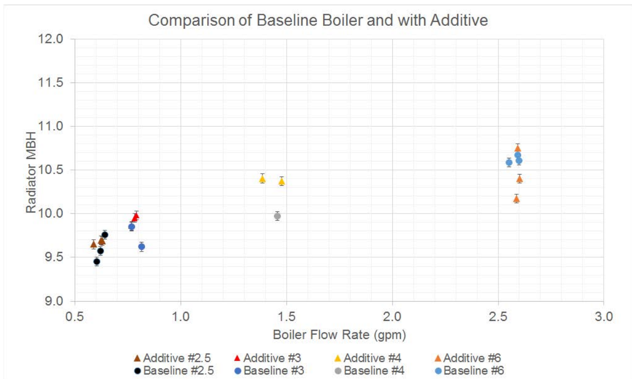
Figure 1: Radiator Output (MBH) Measured for All Test Cases
